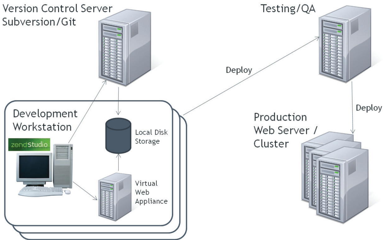
Figure 1 – Best practice application development and deployment model
