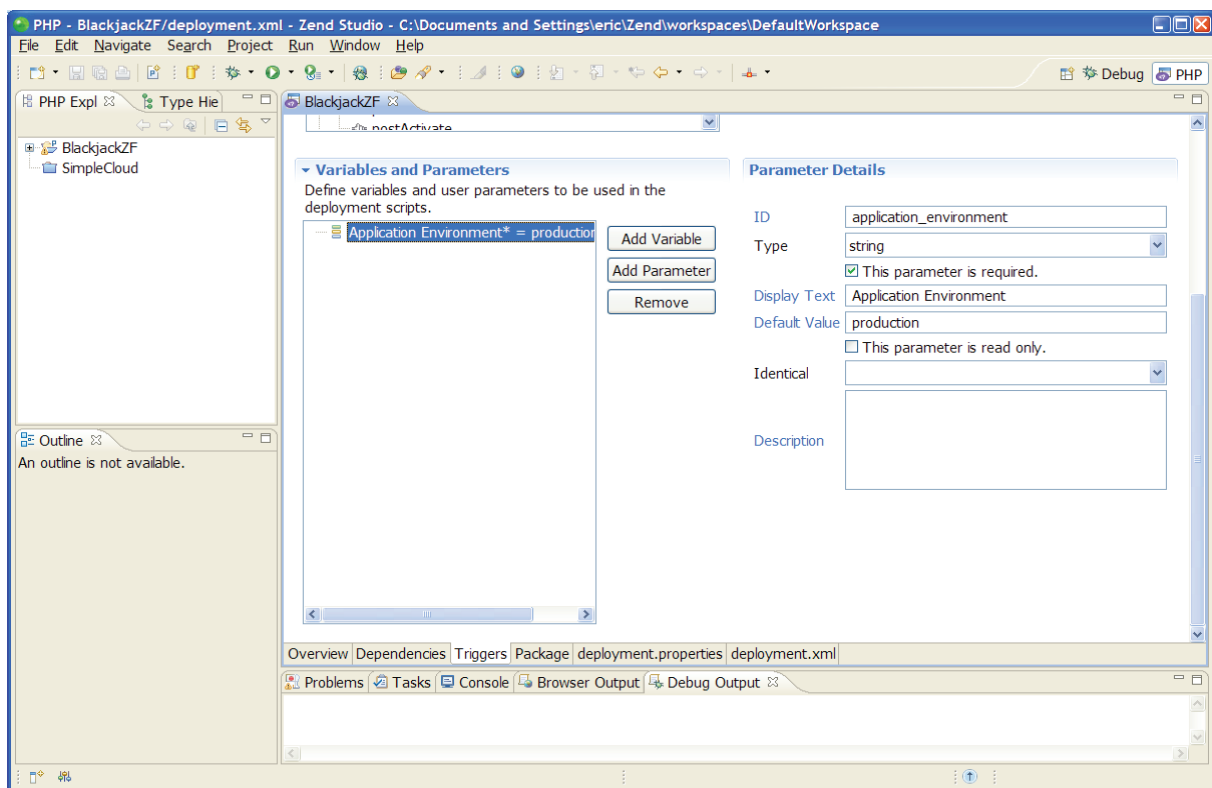
Figure 4 – Defining application environment parameters
