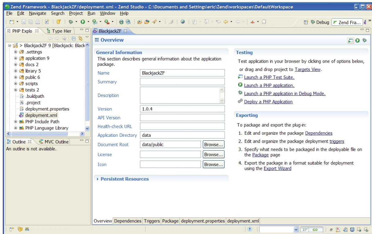
Figure 2 – Deployment configuration in Zend Studio
